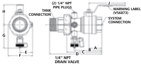
Horizontal Tank Installation with Rolairtrol Air Separator
