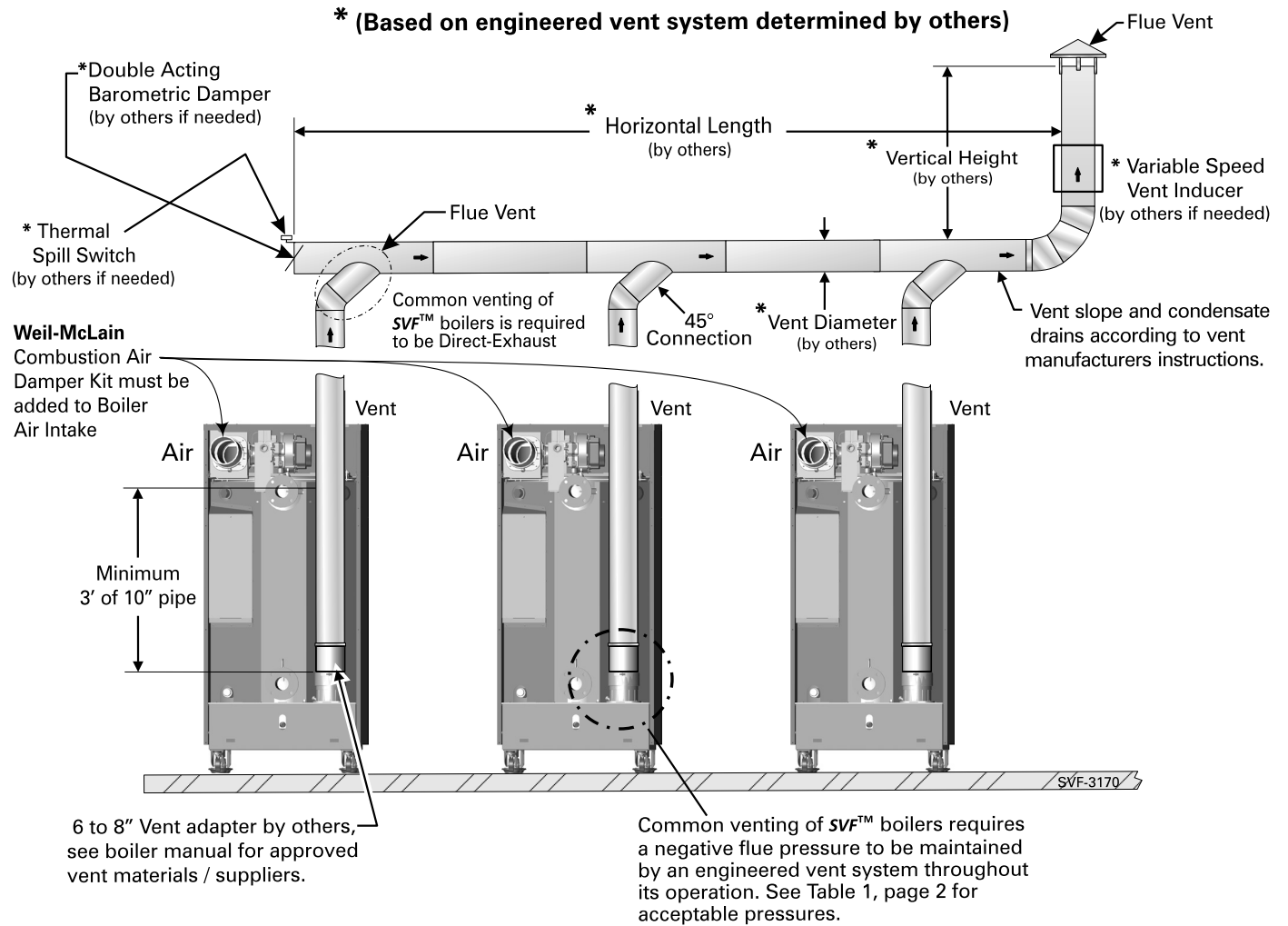
Figure 1 Common vent
