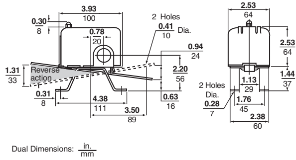
Figure 4: Type DG Dimensions
