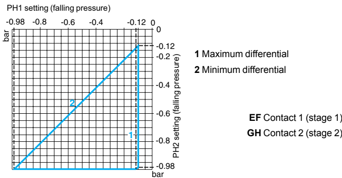
High setting trip points of contacts 1 and 2
