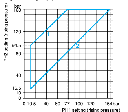
High setting trip points of contacts 1 and 2
