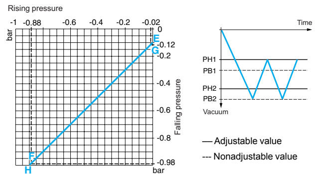
Inherent differential of contacts 1 and 2
