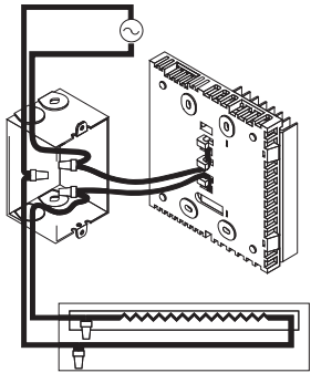
4-wire installation
