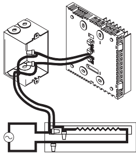
2-wire installation
