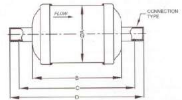
DCH DRIER WITH ODS CONNECTION DIMENSIONS
