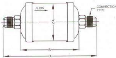
DCH DRIER WITH SAE CONNECTION DIMENSIONS
