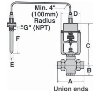
Union ends
