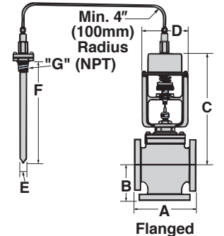
Flanged
