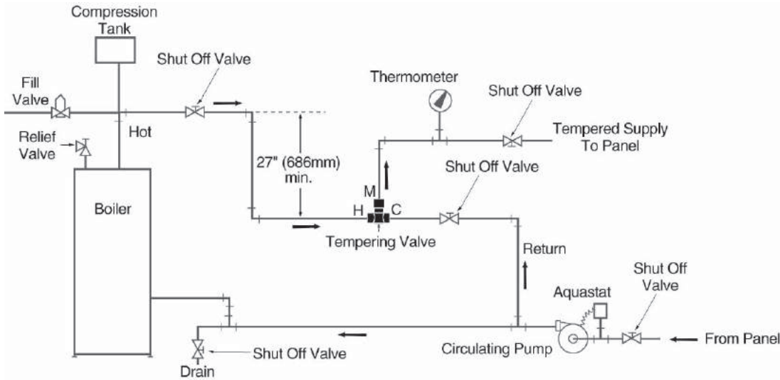
Panel Heating Installation
