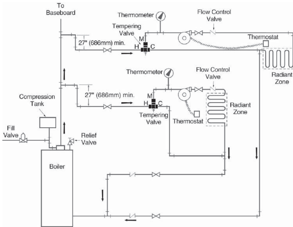
Radiant Heating Installation
