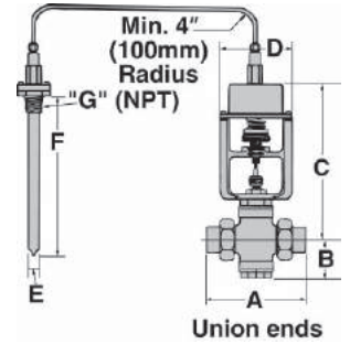
Union ends
