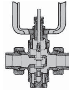
3/4" - 2" NPT
