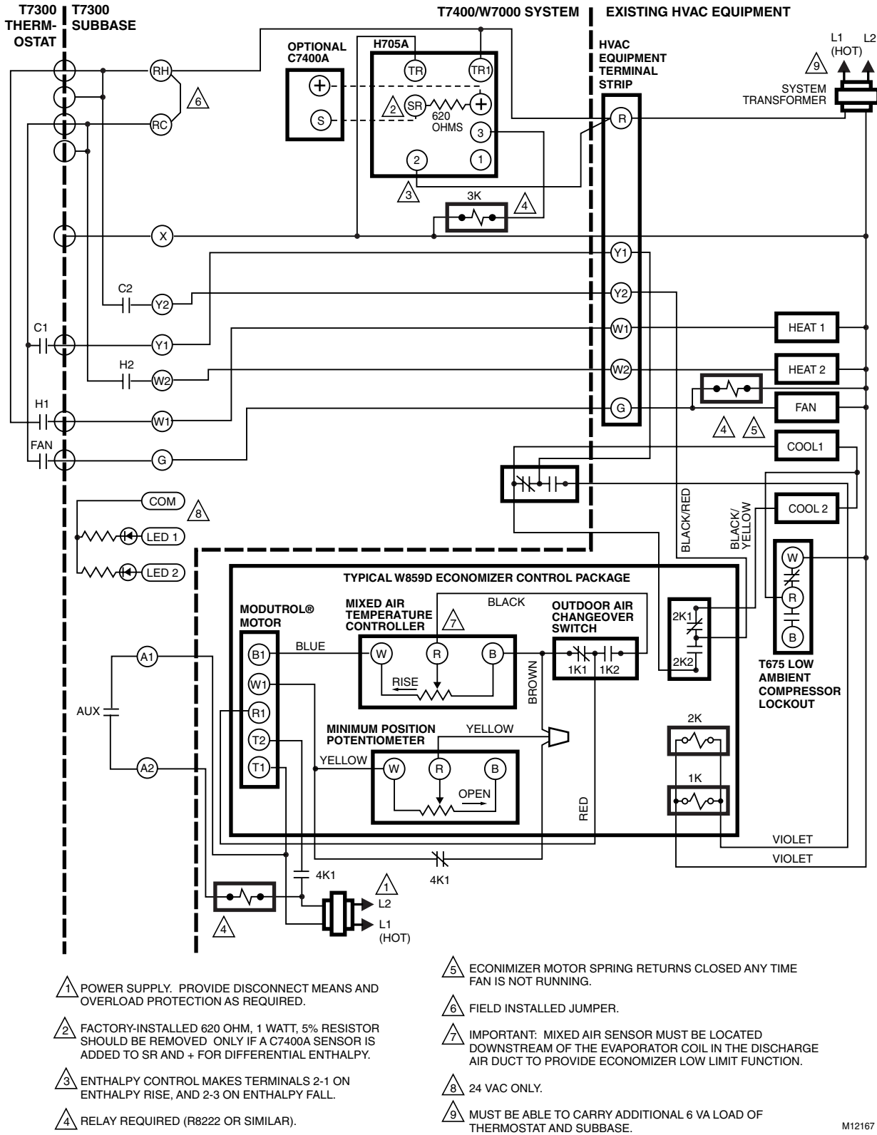
Fig. 5. T7300/Q7300 using W859D Economizer Package with H705A in two-stage heating/two-stage cooling system, defeating economizer minimum position during unoccupied periods.
