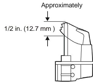
Figure 4: Flame Position
