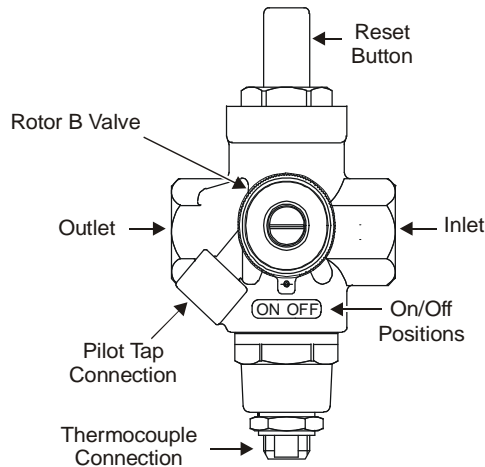
Figure 3: Typical H19 Valve with Rotor Valve
