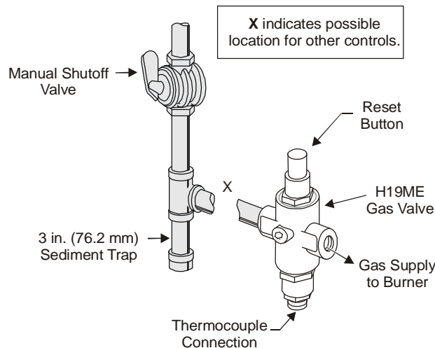
Figure 2: Typical H19ME Installation
