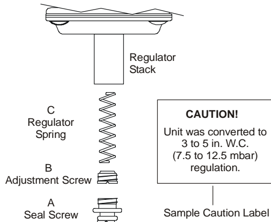
Figure 1: Regulator and Conversion Kit Parts
