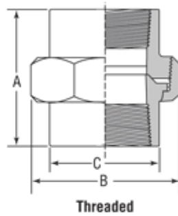
FIGURE 2125: Threaded Union
