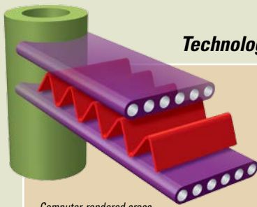
Computer-rendered cross section of MicroChannel Coil
